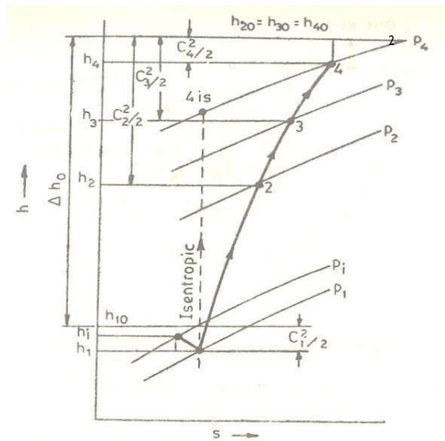
Mollier Diagram of Centrifugal Stage
